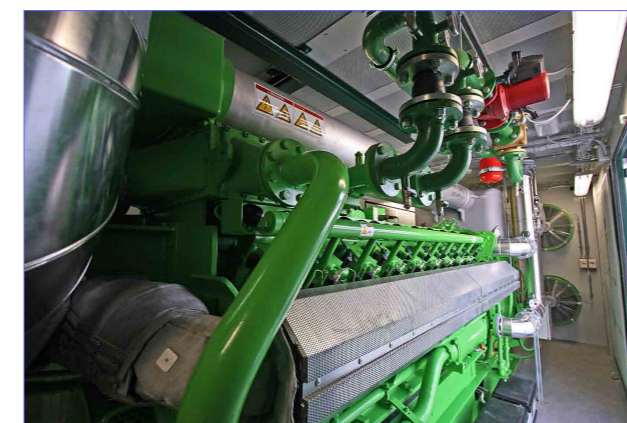
Figure 4: One of the 4 Jenbacher motors, situated in a container purposely designed to house all the process components needed for efficient system management
