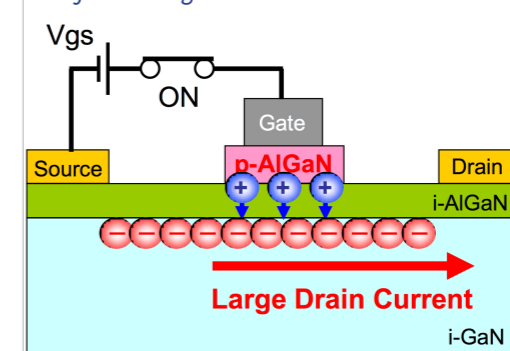
Figure 4(b): Conductivity Modulation when VGS > Vth
