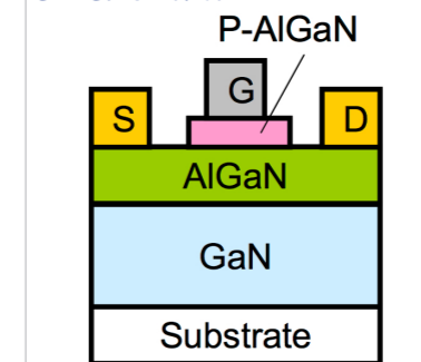
Figure 3(b): P-type AlGaIn for Gate Electrode in Normally Off GIT GaN Structure
