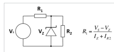
Figure 1: A simple Zener regulator circuit
