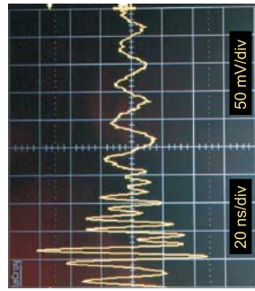
Figure 2a: Power Supply Output Noise 20ns/div.
