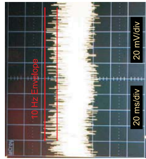
Figure 2c: Power Supply Output Noise 20ms/div.
