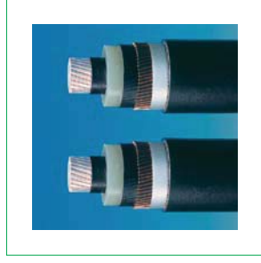
Figure 3: HVDC Light Cables.
