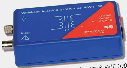
Wideband Injection Transformer B-WIT 100
