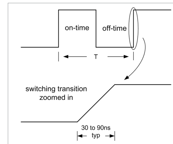
Figure 1: Switching frequency vs. switching transitions
