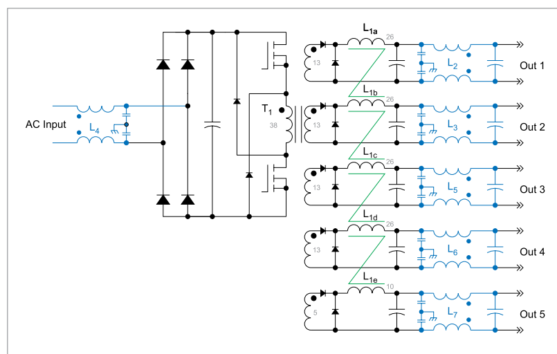
Figure 1: Forward Converter with Five Coupled-Inductor Outputs
