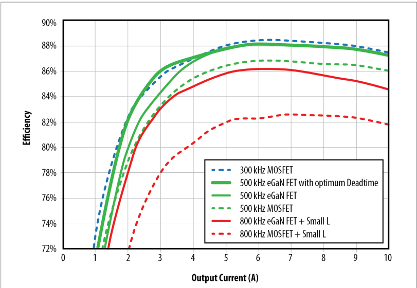
Figure 1: Efficiency comparison between state-of-the-art MOSFETs and eGaN FETs at various frequencies for VIN = 19 V and VOUT = 1.2 V
