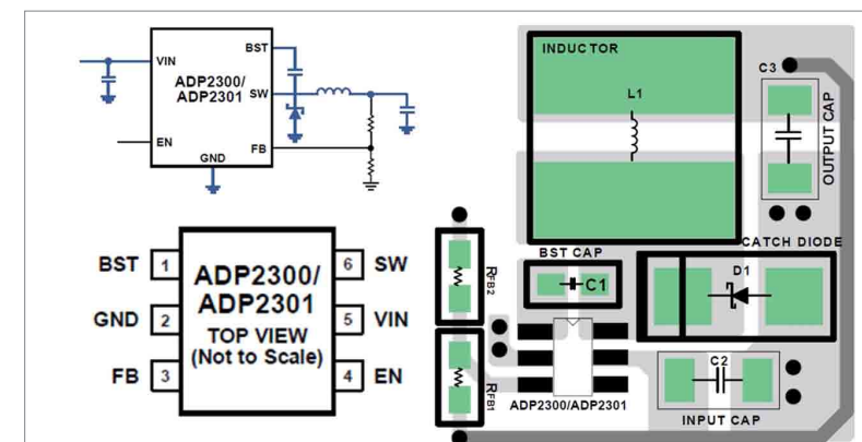
Figure 3: Example of an optimized buck regulator layout
